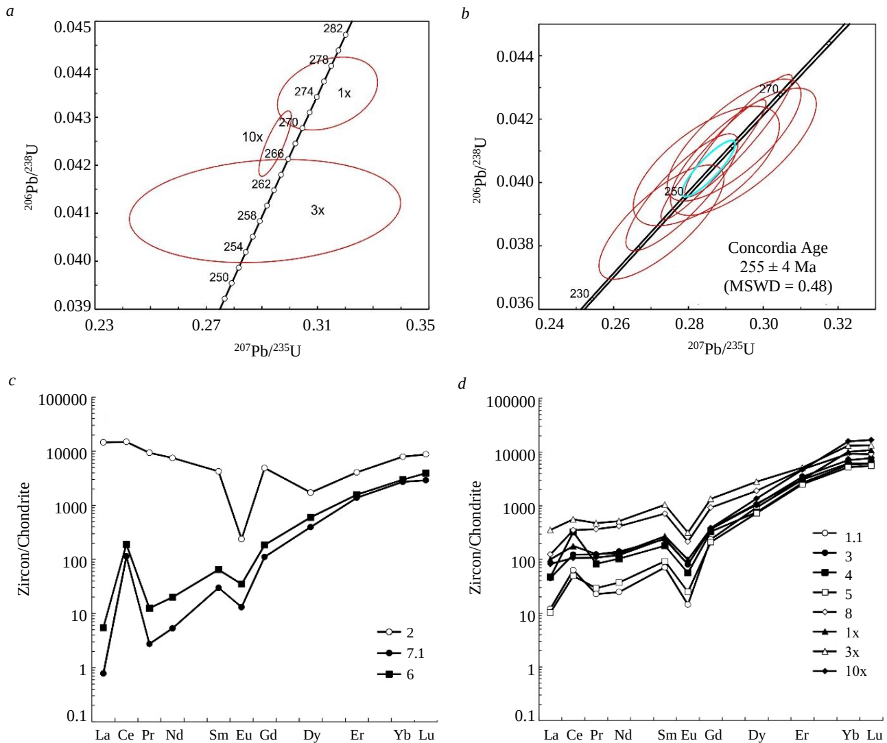
Fig.4. The concordance diagram (a, b) and the REE distribution spectra (c, d), normalized to chondrite CI, for zircons from the third phase granites (sample TH3-1)
