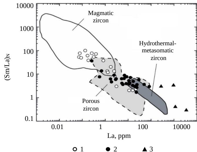
Fig.6. The discrimination diagram for determining zircon genesis. The composition fields are given according to [28, 33, 47].
