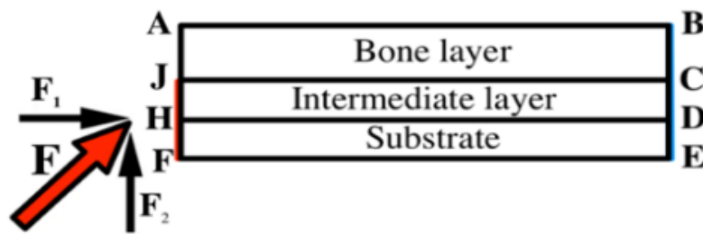
Figure 1 – Boundary and loading conditions
