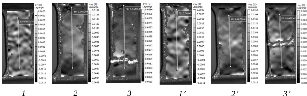
Figure 2 – Patterns of distributions of longitudinal \epsilon_{Y\bar{Y}} relative strains on the surface of the original and modified samples. These patterns correspond to points 1, 2, 3 (Figure 1,a) and 1', 2', 3' (Figure 1, b)
