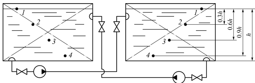
Fig. 1. Scheme for providing additional circulation and density control of technical fluids transported in cargo tanks of specialized vessels
