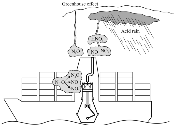
Fig. 1. Nitric acid impact on the environment during the operation of heat engines
