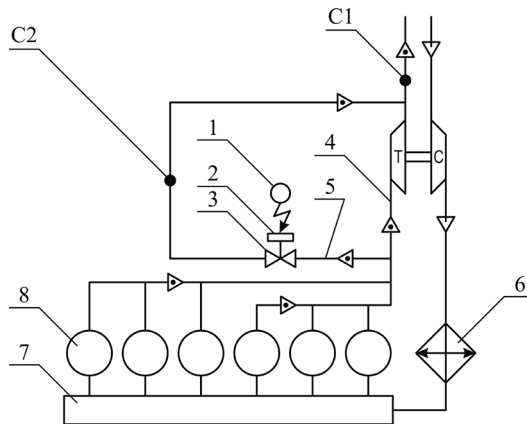
Fig. 3. Schematic diagram of a medium-speed marine diesel engine 6L20 Wartsila with EWG exhaust gas control:
