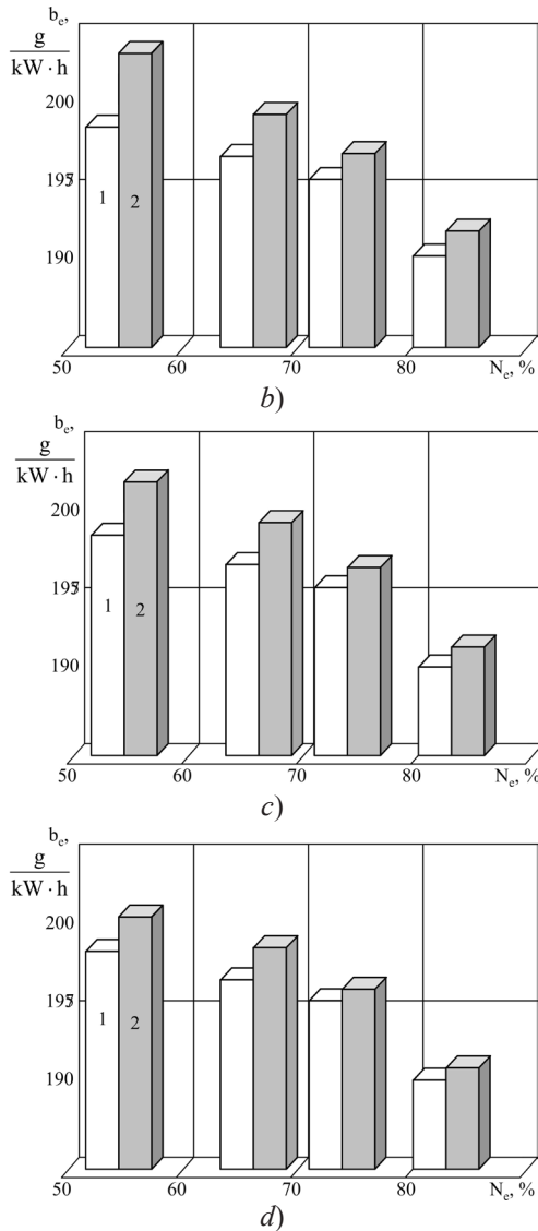
Fig. 5. The dependence of the specific effective fuel consumption b_e of a 6L20 Wartsila diesel engine on the N_e load for different degrees of opening of the gas bypass valve \Delta_{wg} :
