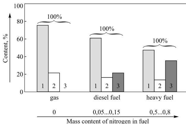
Fig. 2. Nomogram of the distribution of types of NO x for different types of fuel 1 - thermal; 2 - fast; 3 - fuel
