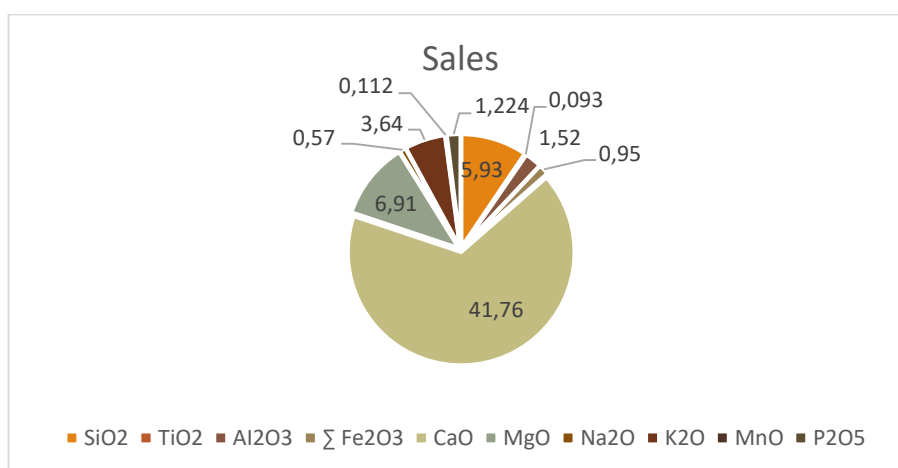
Graph – 1. Chemical composition of ash of Dracocephalum moldavica L
